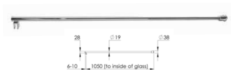
PSG0134 Back to Wall Bracing Kit Chrome
