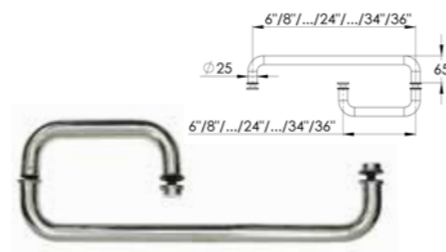
PSG0038 TRound Towel Rail Handle 25 Dia Sizes Available: 6"/8"...24"/34"/36" Chrome
