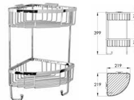
PSG0083 Double Corner Basket Chrome • Matt Black
