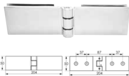
PSG0139 Outward Opening Hinge Chrome
