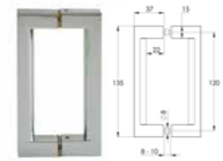
PSG0116 Small Square Handle Chrome
