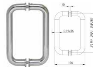
PSG0036 Round D Handle (Note Size options) 19 or 25mm Dia / 220/240mm centres Chrome
