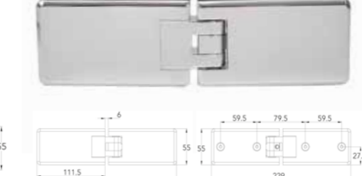
PSG0012 Adjustable inward and Outward Opening Square Glass to Glass Hinge Chrome • Brushed Nickel • Polished Nickel Brushed Brass • Matt Black
