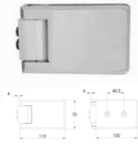
PSG0006 Outward Opening only Square Glass to Profile Hinge Chrome
