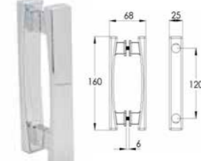
PSG0032 Medium Square Handle 120mm centres Chrome
