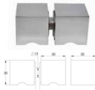
PSG0115 Square Pull Handle Chrome
