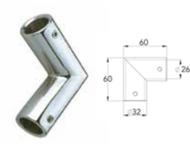
PSG0057 Brace Bar 90° Joint Chrome
