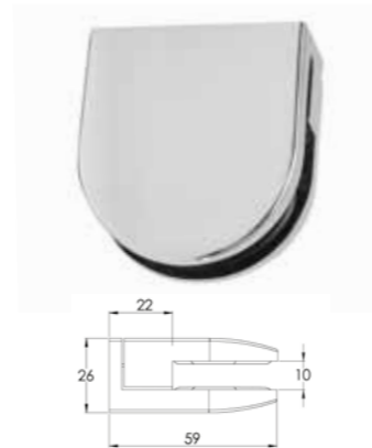
PSG0023 Curved Ceiling Bracket Chrome
