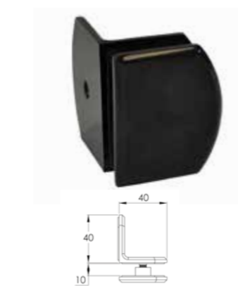
PSG0020 90° Curved Glass to Wall Corner Bracket Matt Black
