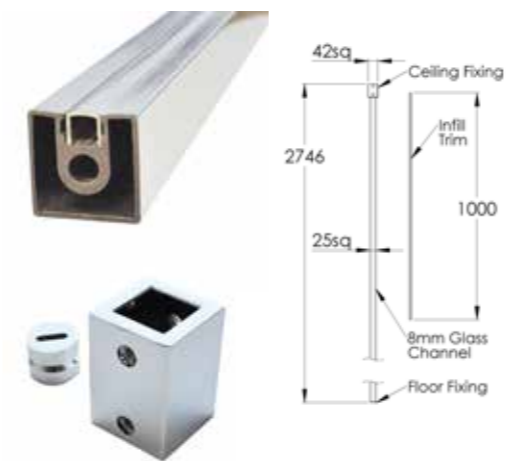
PSG0133 Floor to Ceiling Bracing Kit - Square Chrome • Matt Black
