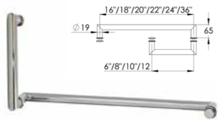
PSG0040 Square Towel Rail Handle 25 Dia Sizes Available: 16"/18"/20"/22"/24"/36" Chrome
