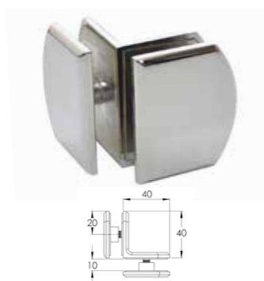
PSG0018 90° Curved Glass to Glass Corner Bracket Chrome
