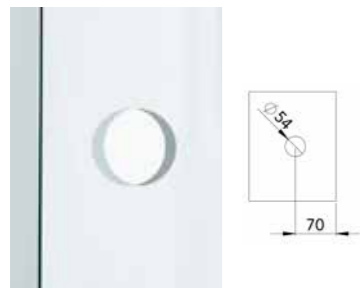
PSG0041 Finger Pull in Glass
