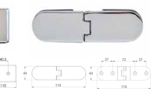
PSG0013 Outward Opening to 90° Hinge Chrome
