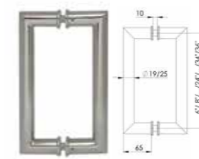
PSG0039 Square Handle 25 Dia / 8" centres (Note Size options) Chrome
