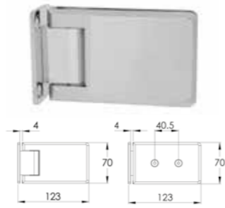
PSG0004 Inward and/or Outward Opening Square Glass to Wall Hinge Chrome
