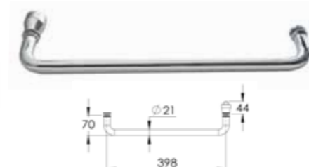
PSG0128 Towel Rail Handle with Rubber Stop 19 Dia Chrome • Matt Black
