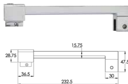
PSG0091 Decem Brace Bar Chrome
