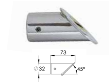
PSG0056 135° Brace Bar Wall Joint Chrome
