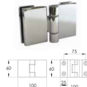
PSG0010 Outward Opening to 90° Bath Screen Hinge Chrome
