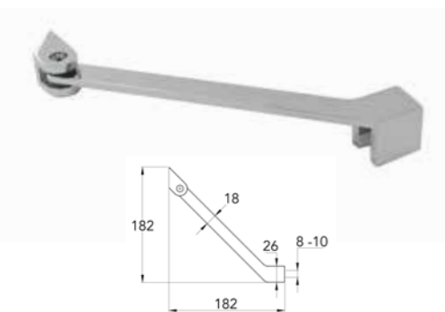
PSG0100 LH Brace Bar Assembly Chrome • Brushed Nickel • Polished Nickel Brushed Brass • Matt Black
