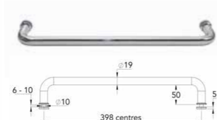
PSG0106 Towel Rail Handle 19 Dia Chrome
