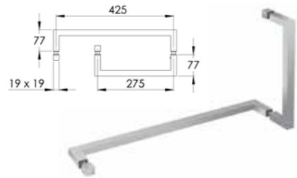
PSG0034 Square Towel Rail Handle 19 x 275 x 425mm Chrome
