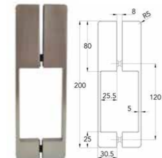
PSG0093 Medium Designer Handle Chrome • Brushed Nickel • Polished Nickel Brushed Brass • Matt Black
