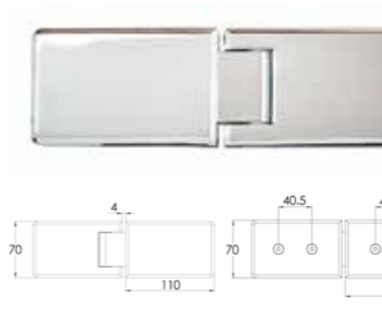
PSG0005 Inward and/or Outward Opening Square Glass to Glass Hinge Chrome
