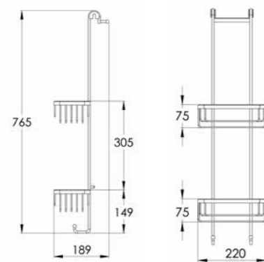
PSG0079 Double Hanging Shower Basket Chrome • Matt Black
