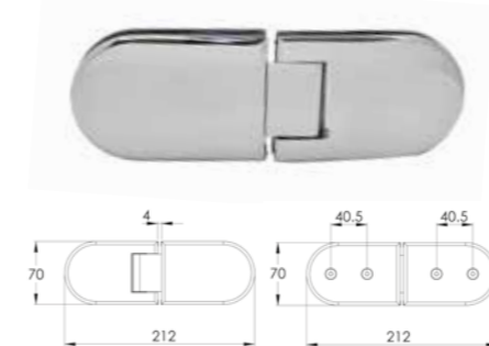
PSG0002 Inward and/or Outward Opening Curved Glass to Glass Hinge Chrome
