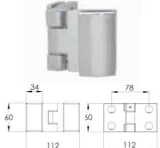
PSG0009 Inward Opening Bath Screen Hinge Chrome
