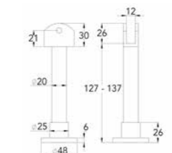
PSG0104 Adjustable Foot Assembly
