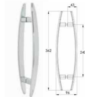
PSG0025 Large Designer Handle 240mm centres Chrome
