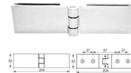
PSG0140 90° Outward Opening Hinge Chrome • Black
