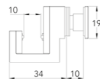
PSG0108 Bottom Guide Assembly Chrome
