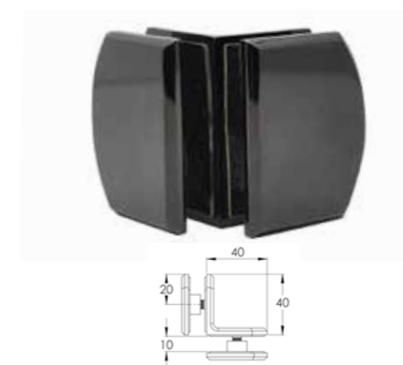
PSG0021 90° Curved Glass to Glass Corner Bracket Matt Black
